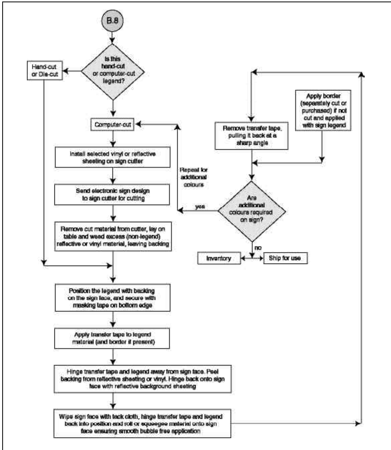
Flowchart B.8 – Legend Application: Direct-applied Copy Metal or Plywood Blanks and Extruded Aluminum Panels
