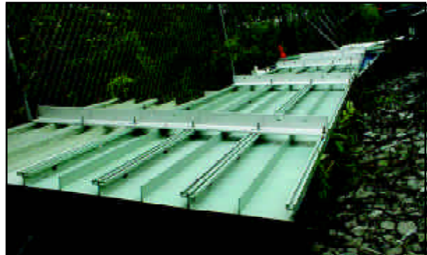
Figure 4.8 – Bolt-together Extruded Panels assembled with T-bars
